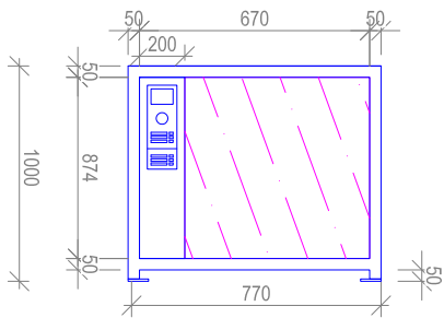
ELEVATION AA
