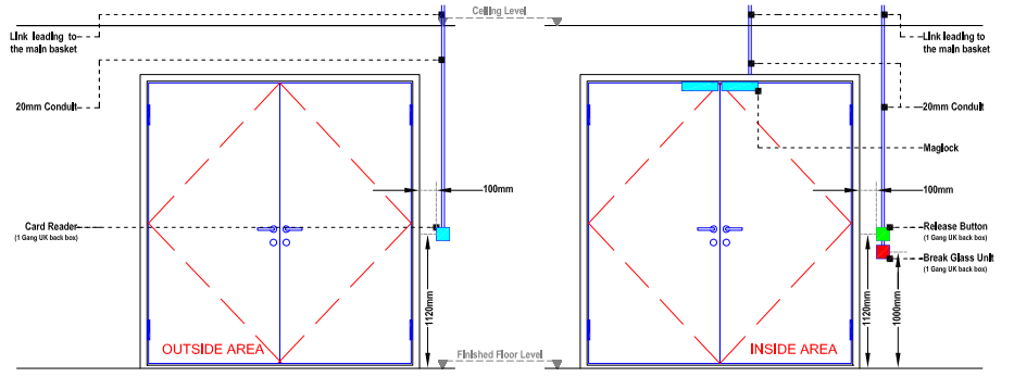
ACCESS DOOR: ACS-GF-014 Bike Parking to Staircase 03
