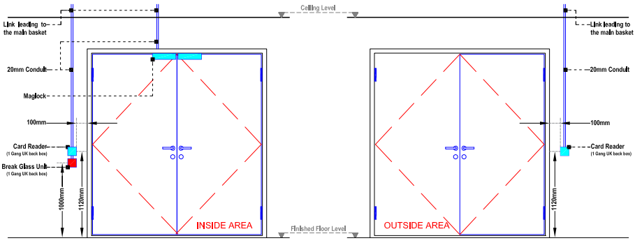
ACCESS DOOR: ACS-GF-004 Service core
