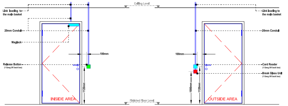
ACCESS DOOR: ACS-GF-013 Service core - Staircase 03
