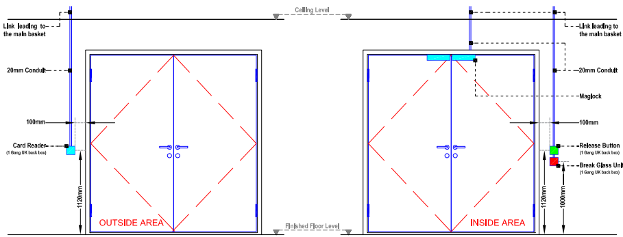
ACCESS DOOR: ACS-GF-005 Staircase 02
