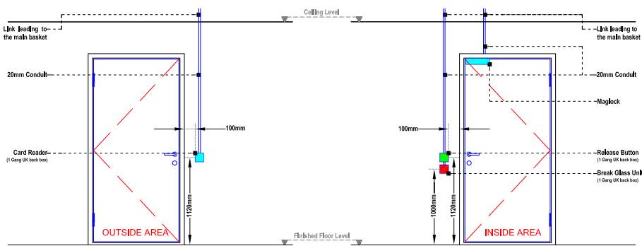
ACCESS DOOR: ACS-GF-011 Lift lobby - Staircase 02
