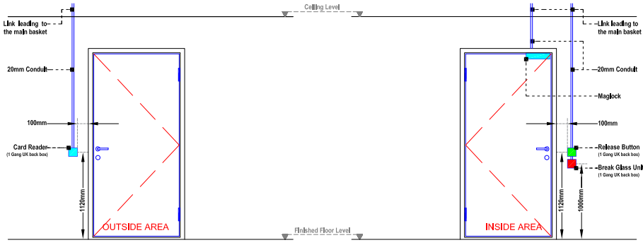
ACCESS DOOR: ACS-GF-003 Access to Lobby near Staircase 03
