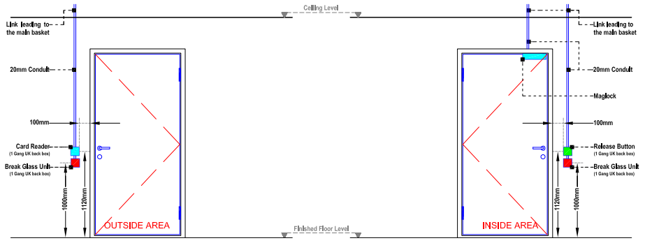
ACCESS DOOR: ACS-GF-015 Emergency exit
