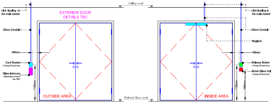
ACCESS DOOR: ACS-GF-002 Staircase 04
