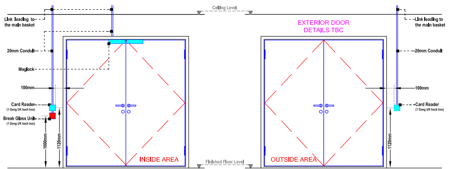
ACCESS DOOR: ACS-GF-017 Emergency exit
